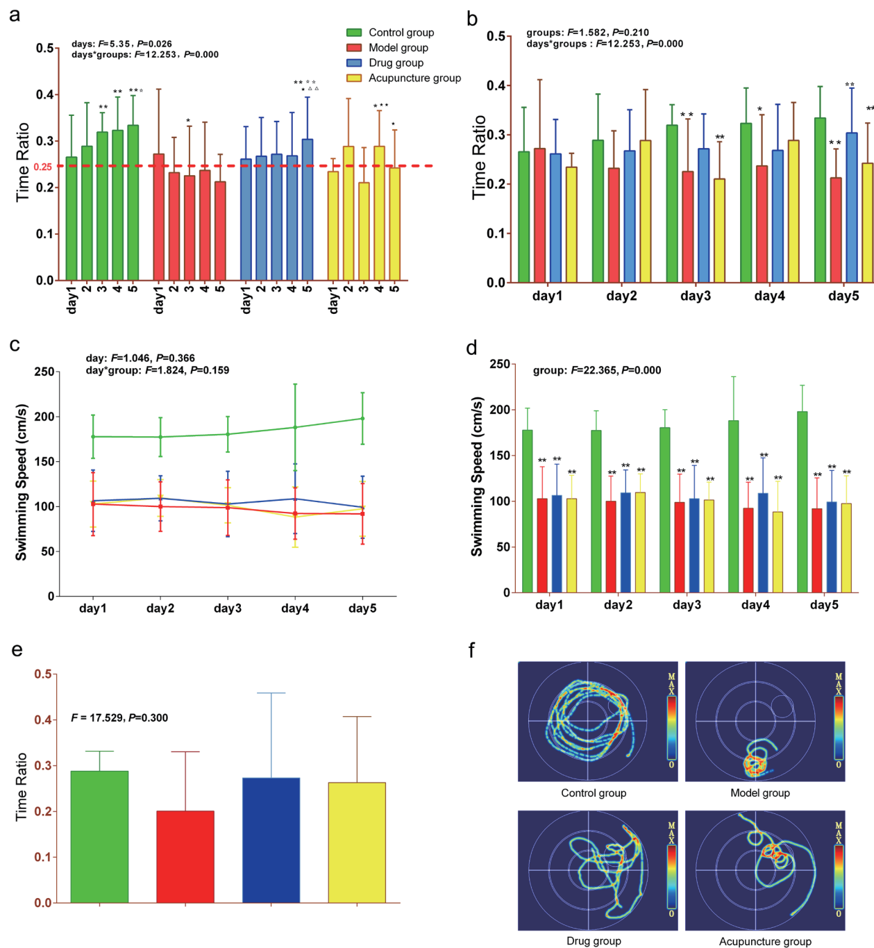
Fig. 1. The effect of acupuncture on the learning and memory abilities of senescence-accelerated prone strain 8 (SAMP8) mice tested by the Morris Water Maze. (a, b) The time ratio that mice spent in the goal quadrant of the total 60 s. (c, d) The swimming speed of mice during the entire test (cm/s). (a, c) In the same group, compared to day 1, * P < 0.05 , ** P < 0.01 ; compared to day 2, ☆ P < 0.05 ; ☆☆ P < 0.01 ; compared to day 3, ★ P < 0.05 ; ★★ P < 0.01 ; compared to day 4, △ P < 0.05 ; △△ P < 0.01 . (b, d) At the same time point, compared to the control group, * P < 0.05 , ** P < 0.01 ; compared to the model group, ☆ P < 0.05 ; ☆☆ P < 0.01 ; compared to the drug group, ★ P < 0.05 ; ★★ P < 0.01 . (e) The time ratio of mice spent in the spatial exploration test. (f) The strategy that mice in different groups used to find the platform in the spatial exploration test. Control group, n = 11 ; Model group, n = 10 ; Drug group, n = 11 ; Acupuncture group, n = 10 .
